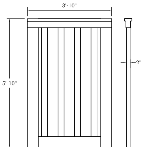
STANDARD 4' X 6' WALK GATE PANEL
